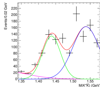
Figure 8: M(K^*\bar{K}) , J = 2 from PWA.
