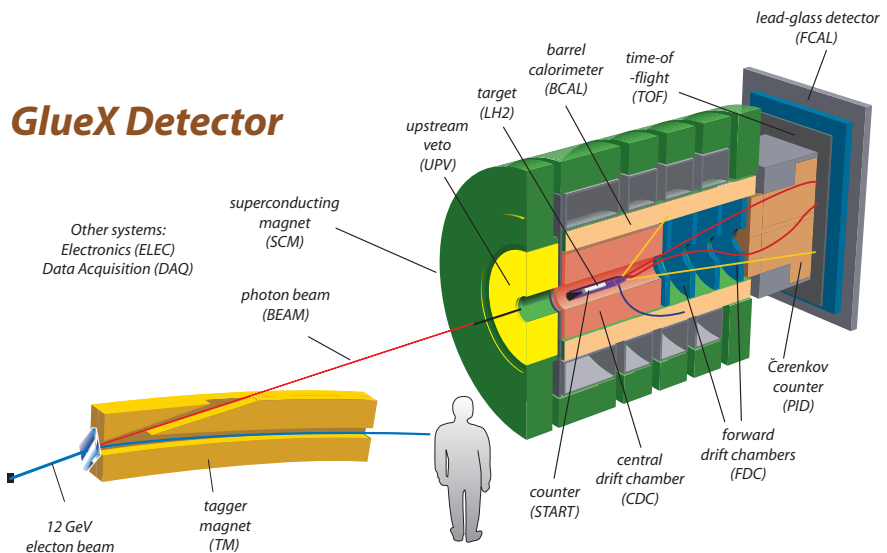
Figure 2: Diagram of Hall D and the GlueX detector.
