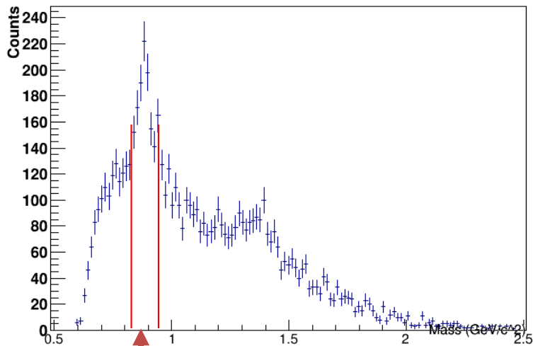
Counts versus invariant K - Pi 0 mass
