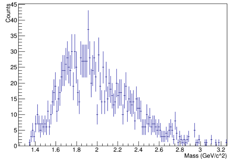
Counts versus invariant K + K + mass
