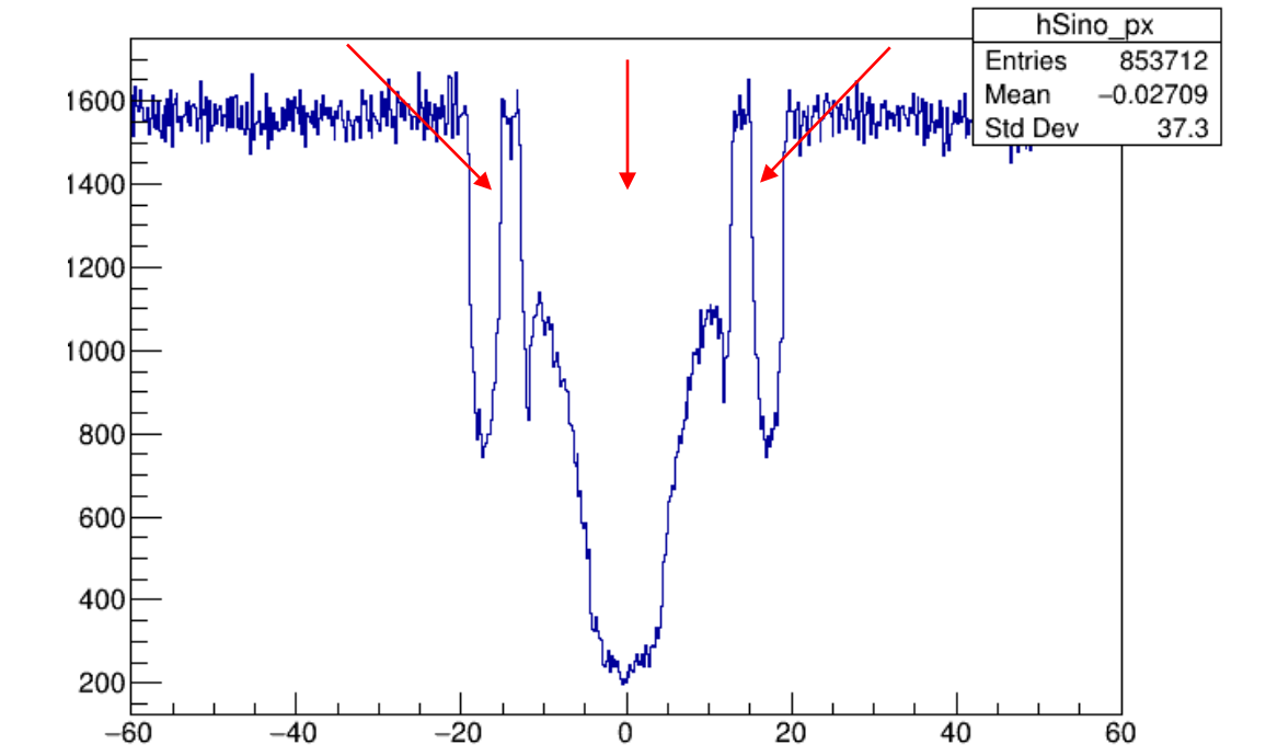
Figure 4: Occupancy of detector hit position for an angle of 90°.
