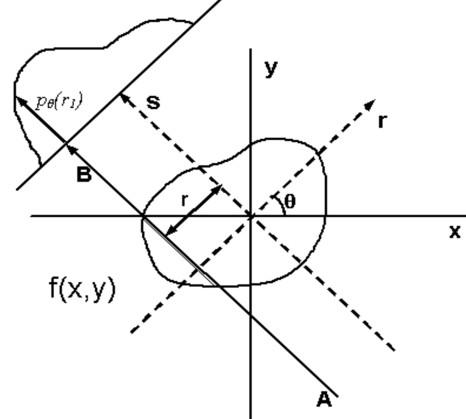
Figure 1: Parallel beam geometry used in tomographic reconstruction.
